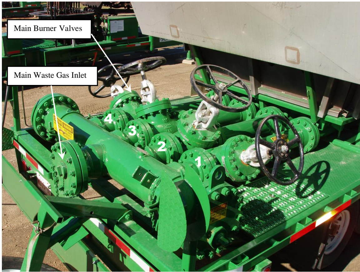
FIG. #2 MAIN WASTE GAS MANIFOLD AND BURNER VALVE LAYOUT
