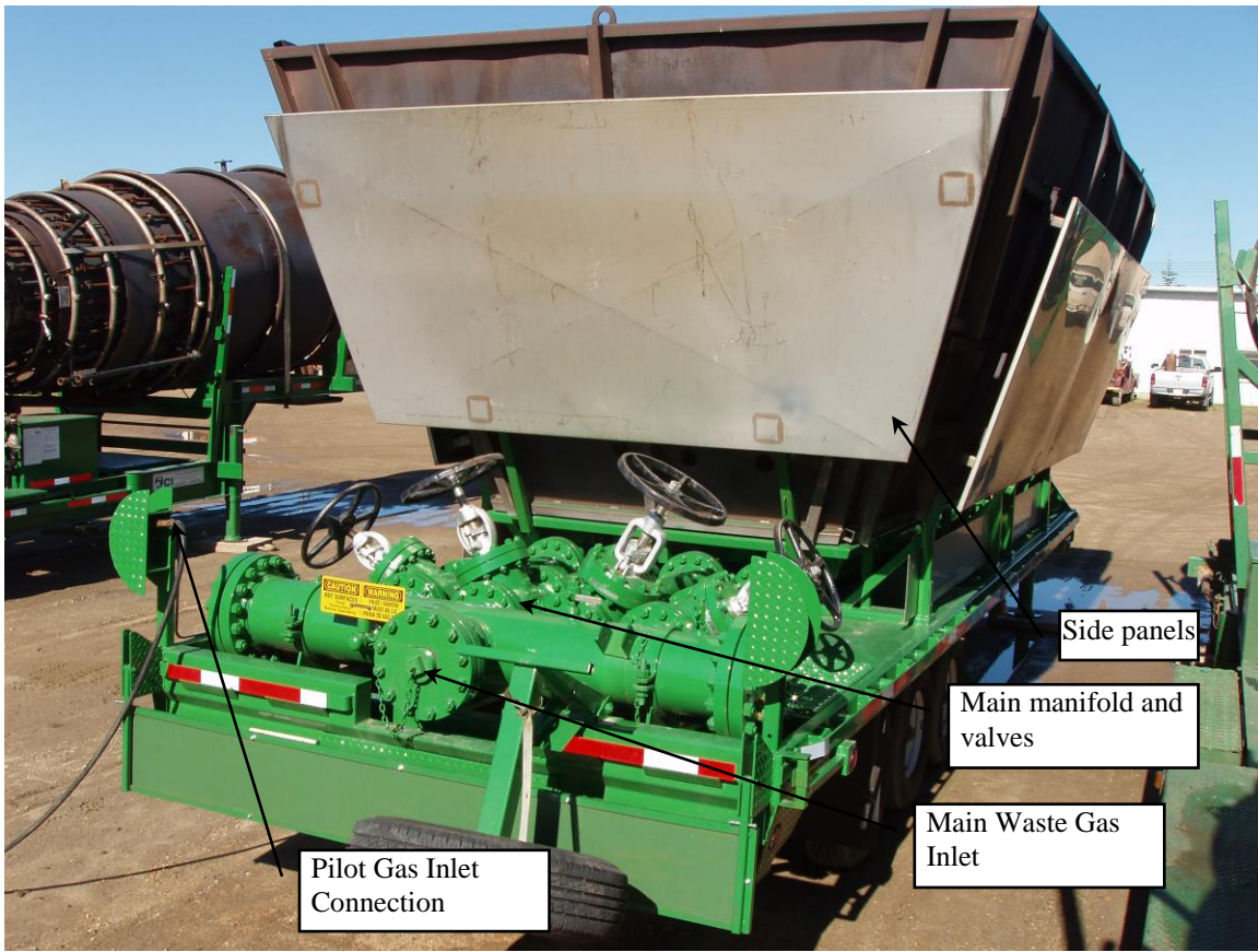
FIG. # 1 TCI 7500 UNIT CONFIGURATION AND MAJOR COMPONENTS
