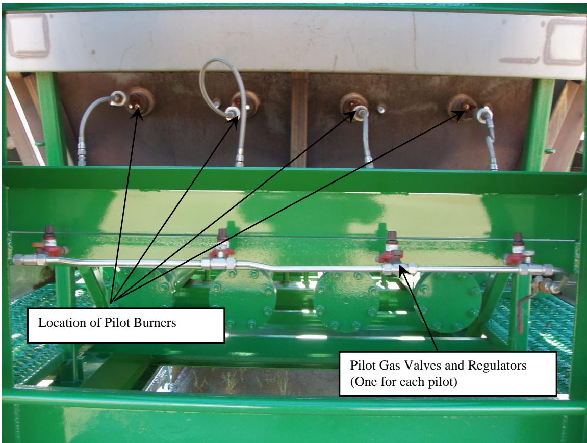
FIG. # 3 PILOT BURNER LOCATIONS (AT FRONT END OF TRAILER)
